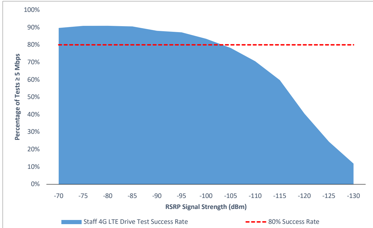
Figure 24. Percentage of Successful 4G LTE Staff Drive Tests by RSRP
